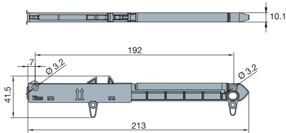
Titusoft mechanism
