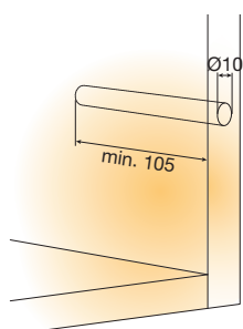
Drilling pattern
