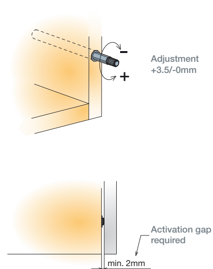
Door gap adjustment
