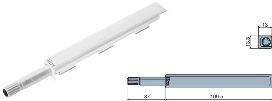
Push Latch S3 routed
