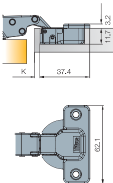
Technical details
