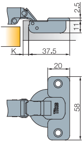
Technical details
