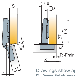
Mounting details
