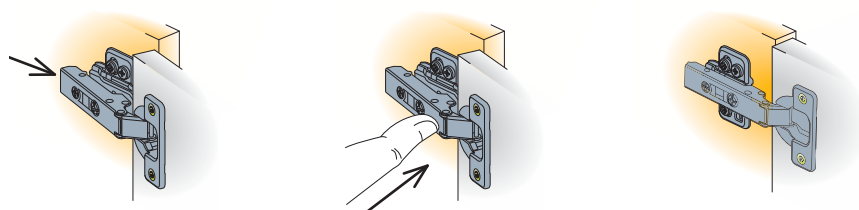
front assembly
