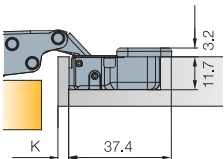
Technical details
