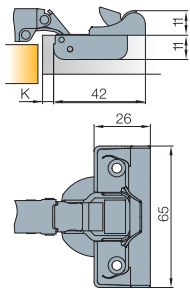
Technical details
