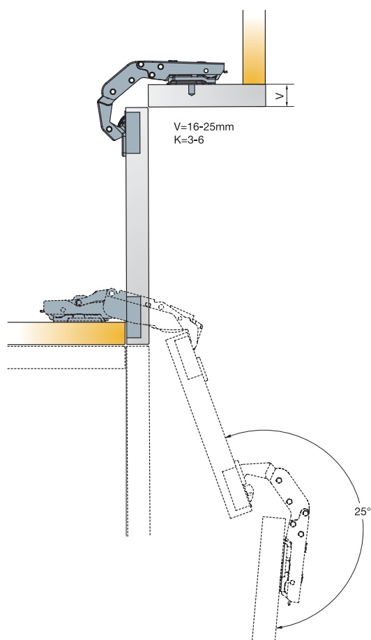
Push opening
