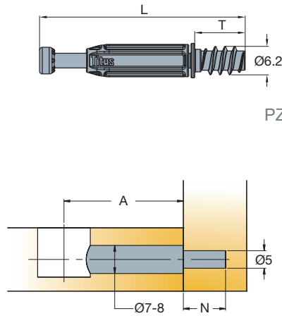
Technical and mounting details
