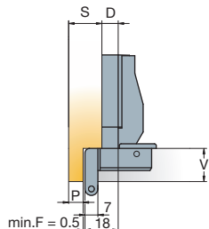
Drawing shows application on D=6mm mounting plate
