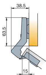
Drawing shows application on D=0mm mounting plate
