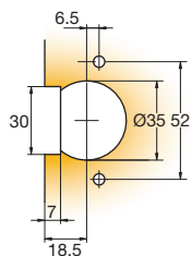
Drawing shows application on D=6mm mounting plate
