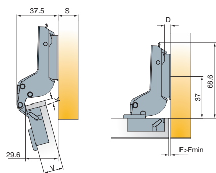
Drawings show application on D=2mm mounting plate
