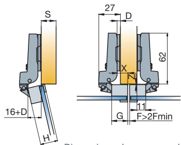
Dimensions shown on m.pl. D=0mm
