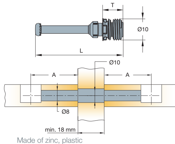
Quickfit dowel For back-to-back application Ø10mm
