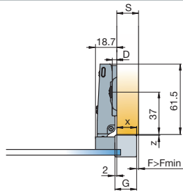
Dimensions shown on m.pl. D=0mm
