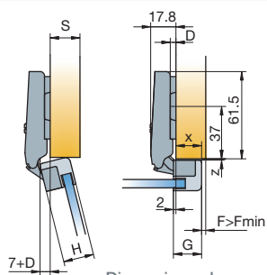
Dimensions shown on m.pl. D=0mm
